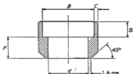
Welding Boss - Socket Weld.
