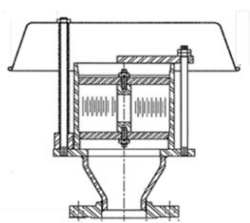
Flame Arrestor
