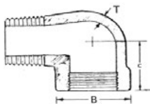
Street Elbow
