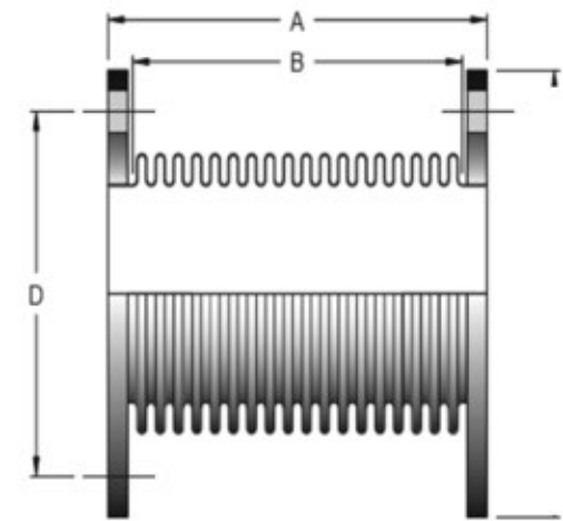
Bellow – Expansion Joint
