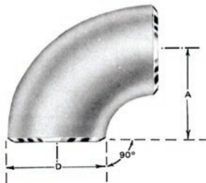
90° Short Radius Elbow
