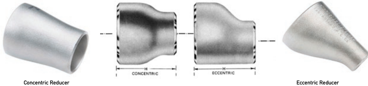
Concentric Reducer
