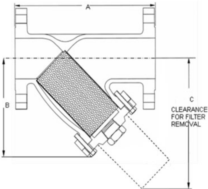
Y-Type Strainer
