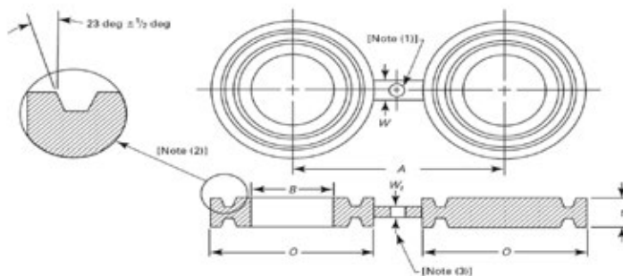
Ring Joint Facing Figure-8 Blanks
