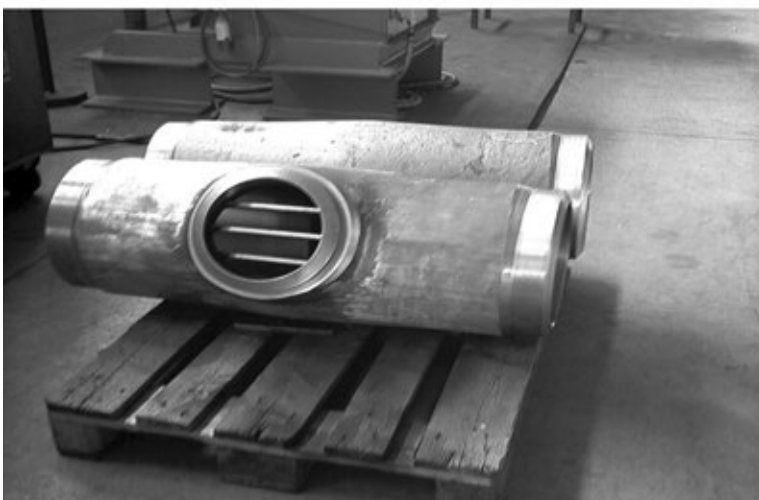
Barred Tee
